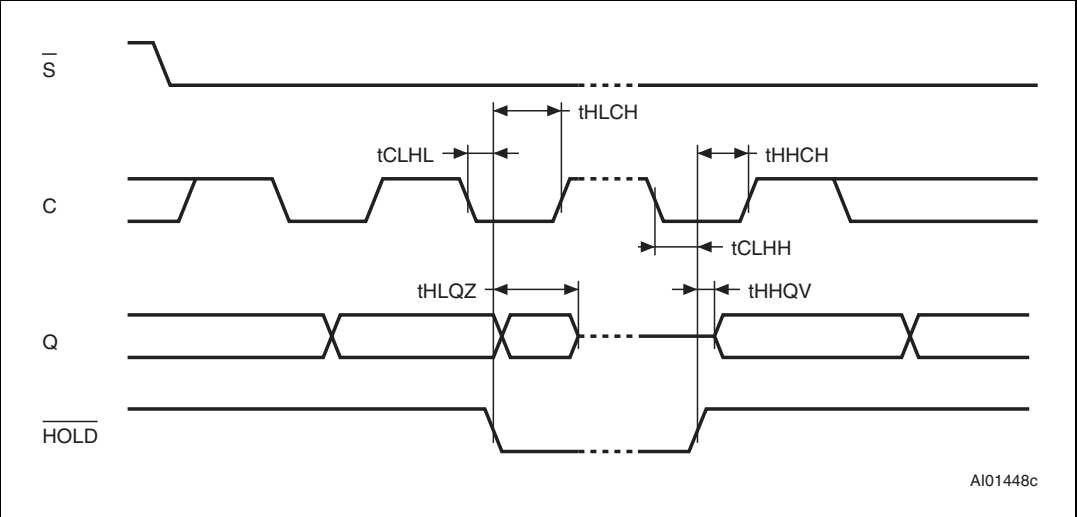
Figure 17. Hold timing
